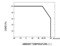
Derating Curve
