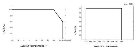
Derating Curve
