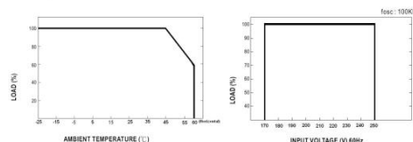
Derating Curve
